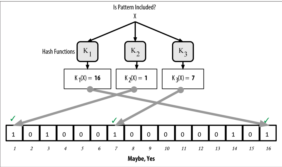
Figure 6-11. Testing the existence of pattern “X” in the bloom filter. The result is probabilistic positive match, meaning “Maybe.”
