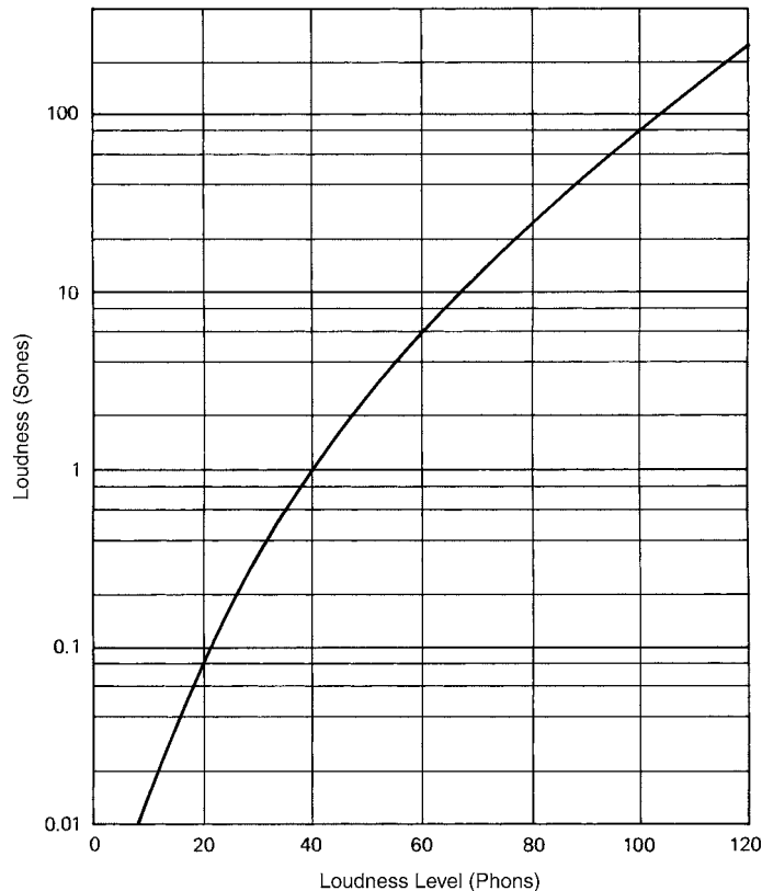
FIGURE 3.16 Loudness function showing the relationship between loudness (in sones) and loudness level (in phons).
