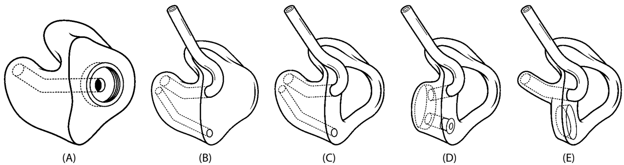
FIGURE 14.7 Five types of earmolds, showing (A) receiver type for use with external transducer, vented to reduce low frequencies; (B) shell type for severe impairment; (C) skeleton; (D) open-bore canal for enhanced high frequencies; (E) minimum contact mold for reduced occlusion effect. (Courtesy of Westone Laboratories, Inc.)
