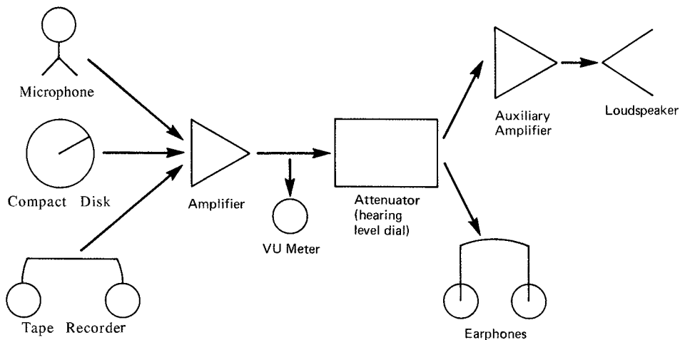
FIGURE 3.24 Block diagram of the speech circuit of a diagnostic audiometer.
