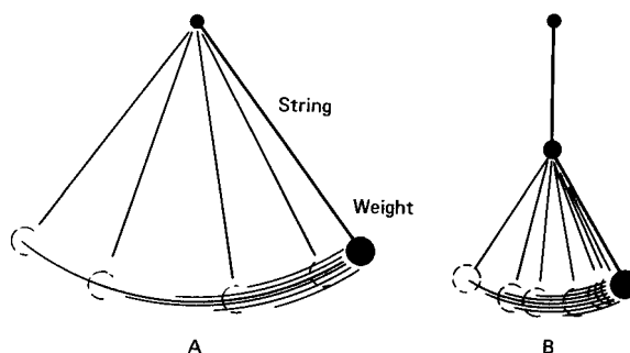
FIGURE 3.7 Effects of the length of a pendulum on the frequency of the vibration. Given a length of string, the weight at the end will swing back and forth a specific number of times per second. If the string is shortened (B), the weight will swing faster (increase in frequency).
