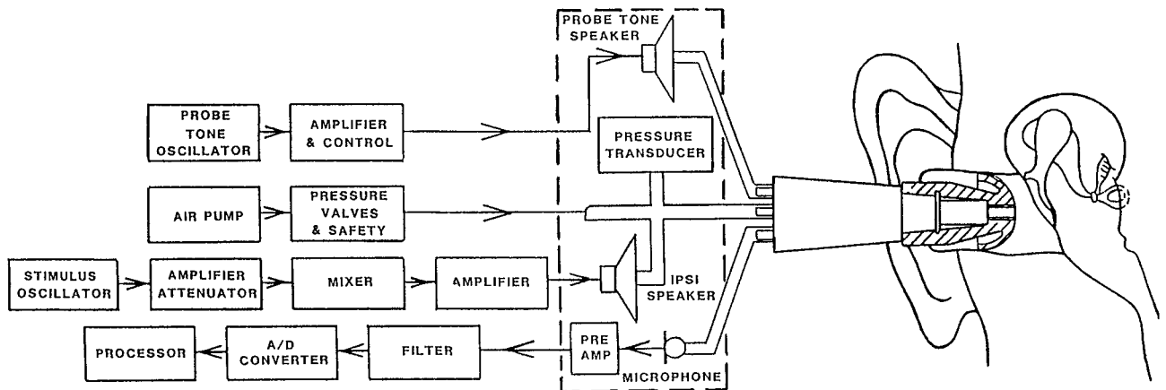
FIGURE 7.2 Diagram of an electroacoustic immittance meter showing its three primary components: a speaker to present a tone to the ear, a microphone to measure the intensity of the tone as it is reflected from the tympanic membrane, and an air-pressure pump to vary the pressure within the external auditory canal. (Courtesy of Grason-Stadler Co.)
