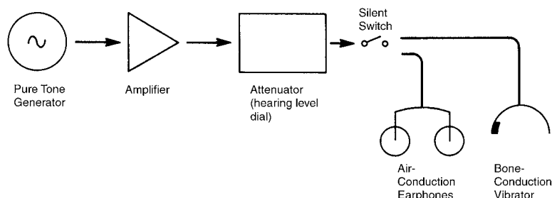
FIGURE 3.18 Block diagram of a pure-tone audiometer.
