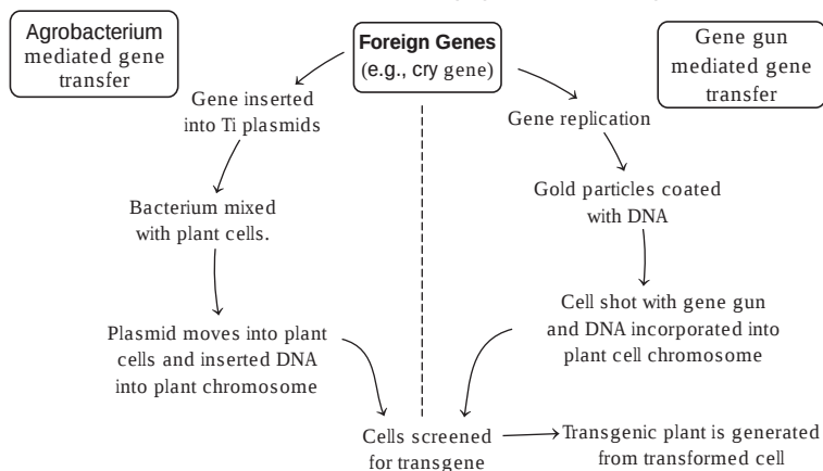
Generation of Bt cotton
