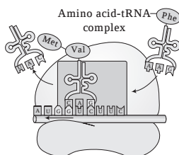
Elongation of polypeptide chain
