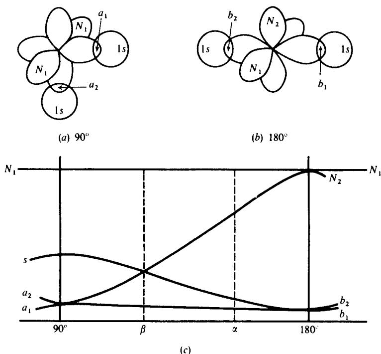
Figure 6.16 Orbital pictures for an AH_2 molecule where the AH bonds are (a) at 90^\circ and (b) at 180^\circ . In (c) is shown qualitatively the change in energy of the various orbitals as the bond angle changes from 90 to 180^\circ . (Adapted, with kind permission of the author, from A. D. Walsh, J. Chem. Soc., 1953, p. 2262.)
